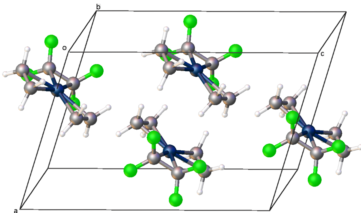
Bis(ethylene)(Tetrafluoroethylene) Platinum
